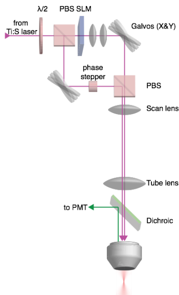
Implementation of aberration correction with in a nonlinear microscopy setup.
