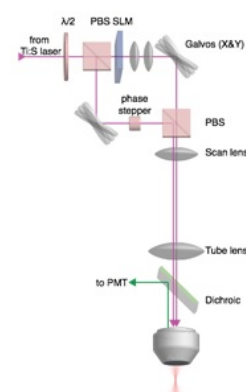
Implementation of aberration correction within a nonlinear microscopy setup.
